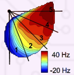
Spindle firing rate differences between two muscles recorded in frog wipe reflex, then used in a neuromechanical model
