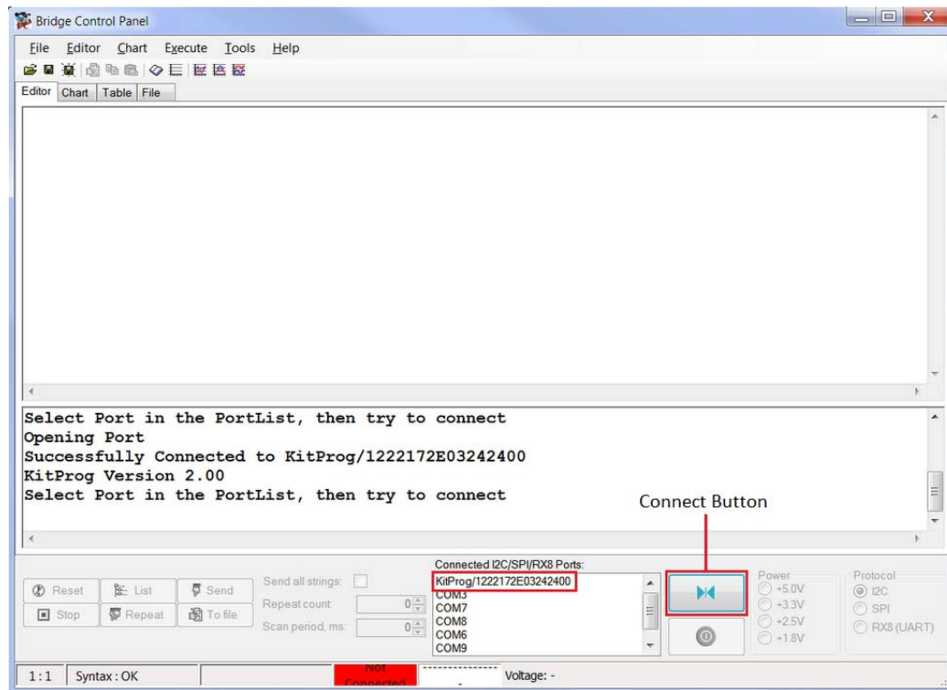
Figure 3-11. Bridge Control Panel
