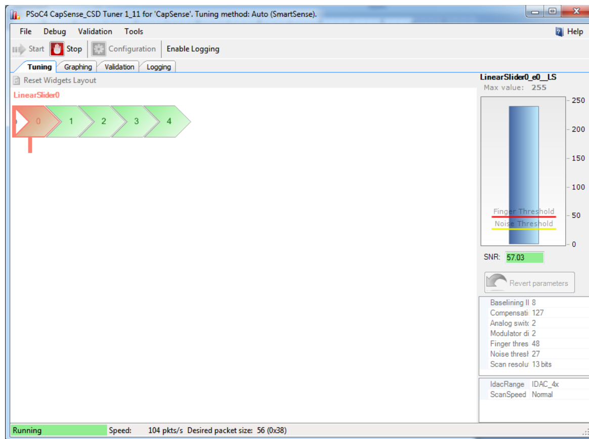
Figure 5-26. Sensor Tuning
