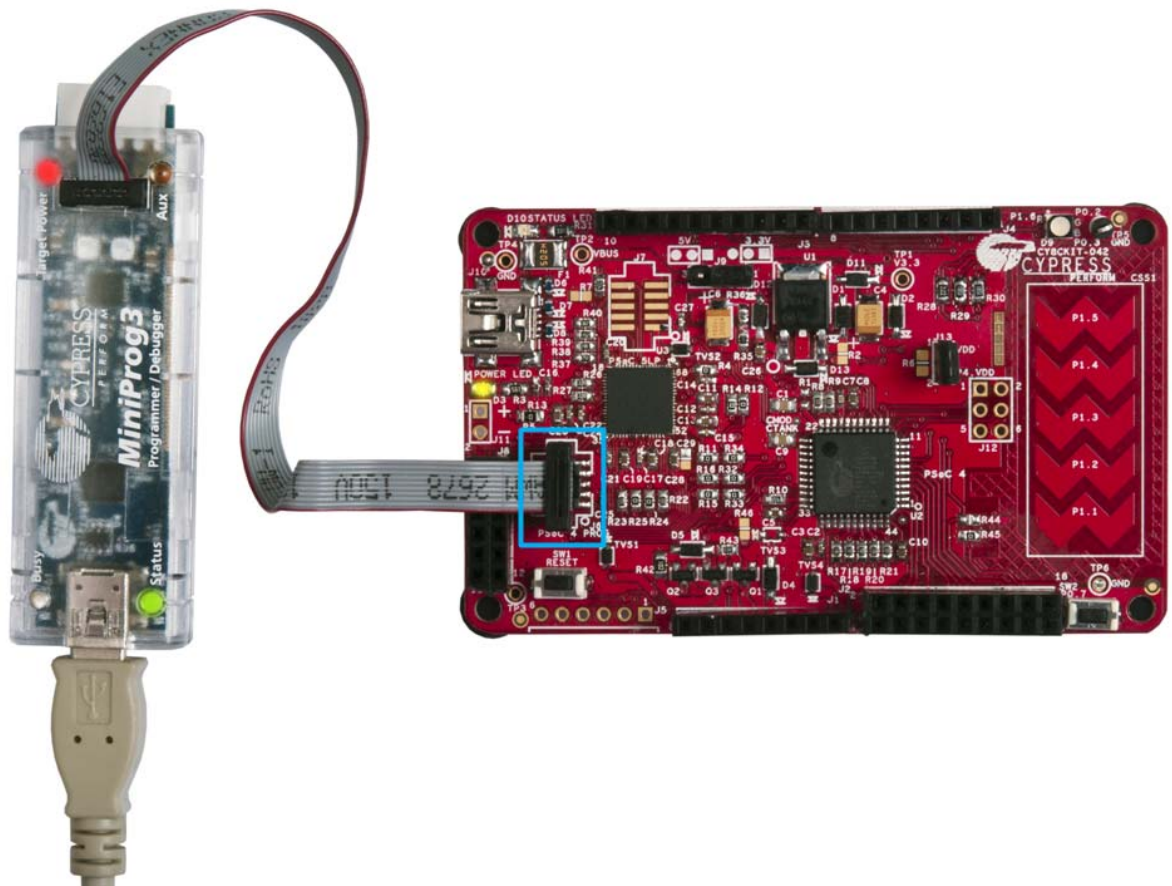
Figure 3-8. PSoC 4 Programming/Debug Using MiniProg3
