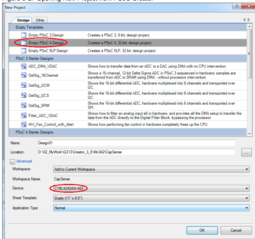
Figure 6-1. Opening New Project from PSoC Creator
