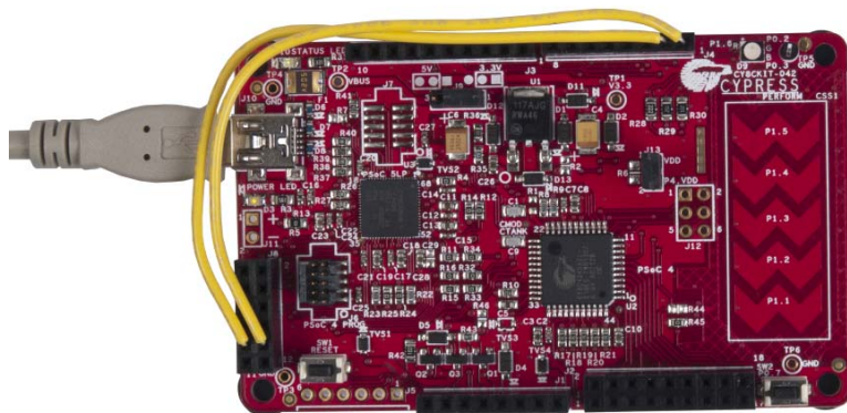
Figure 6-8. UART Connection Between PSoC 4 and PSoC 5LP
