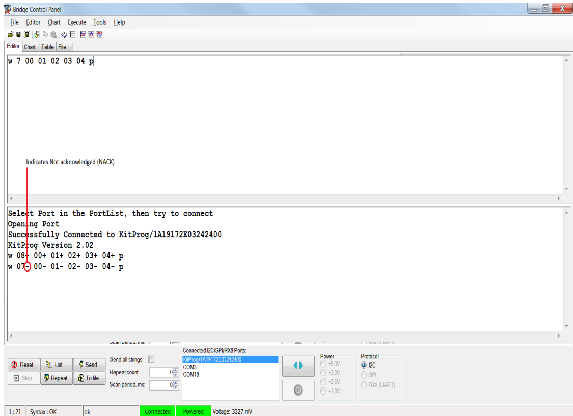
Figure 6-28. NACK Indication in BCP
