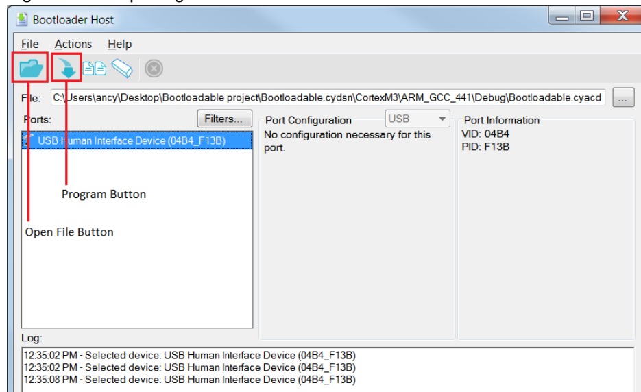
Figure 6-41. Opening Bootloadable File from Bootloader Host Tool
