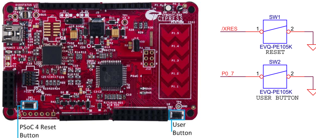
Figure 4-18. Push Buttons
