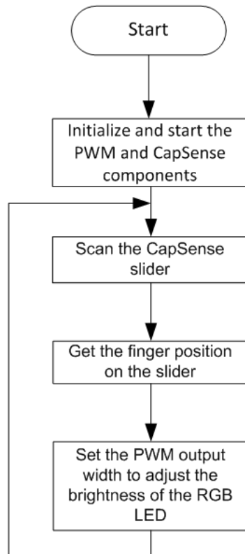
Figure 5-19. CapSense Project Flow Chart
