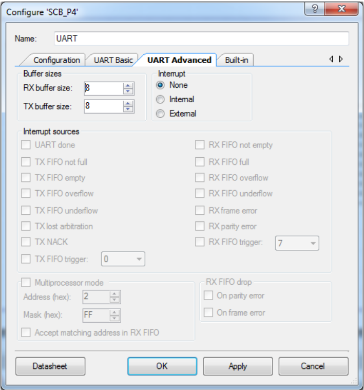
Figure 6-6. UART Advanced Configuration Window
