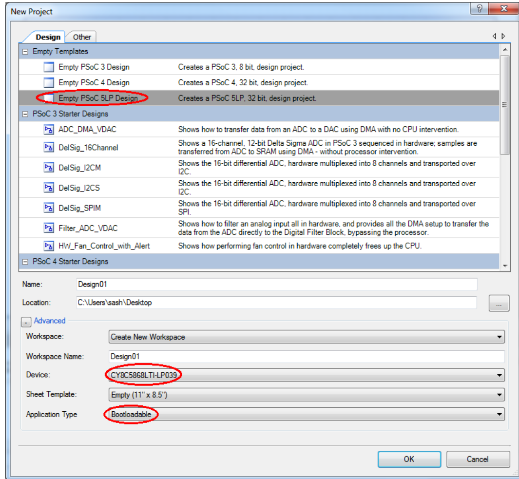
Figure 6-32. Opening New Project in PSoC Creator
