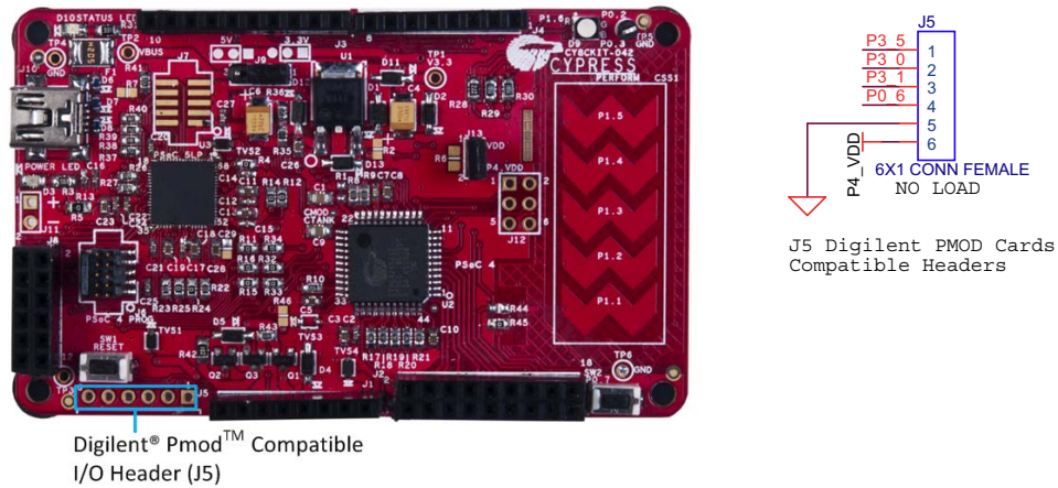
Figure 4-11. Digilent Pmod Interface
