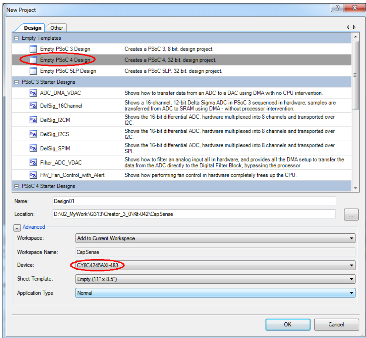
Figure 6-19. Opening a New Project in PSoC Creator
