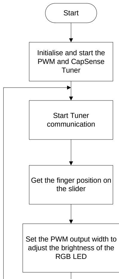
Figure 5-20. CapSense with Tuning Flow Chart
