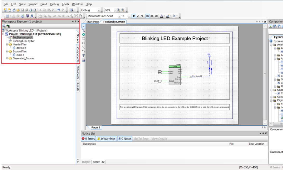
Figure 2-7. Workspace Explorer
