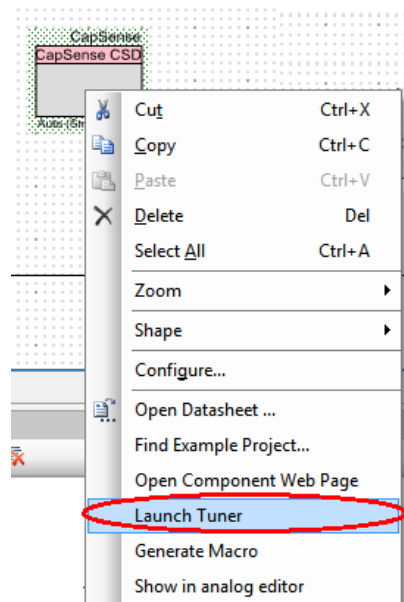
Figure 5-22. Launch Tuner
