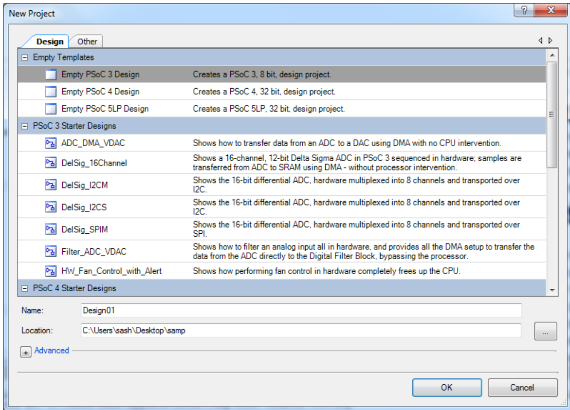
Figure 2-4. Starter Designs
