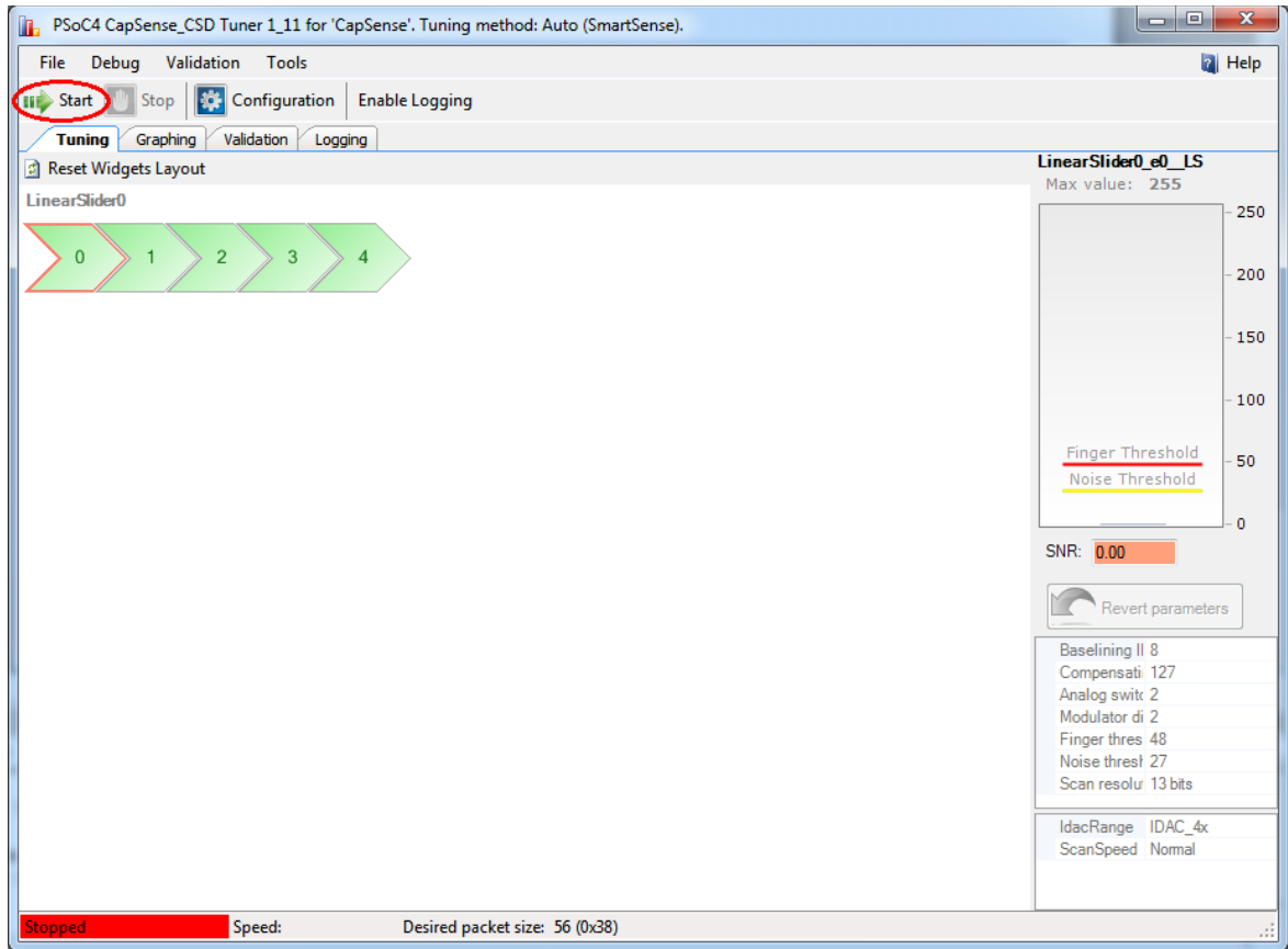
Figure 5-25. Start Communication
