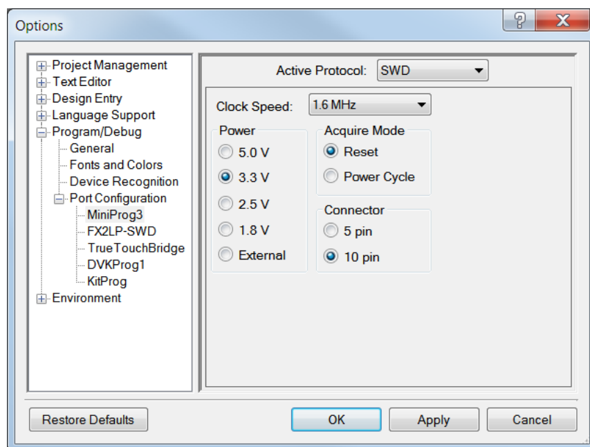
Figure 3-9. MiniProg3 Configuration
