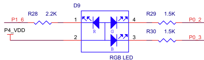
Figure 4-17. RGB LED
