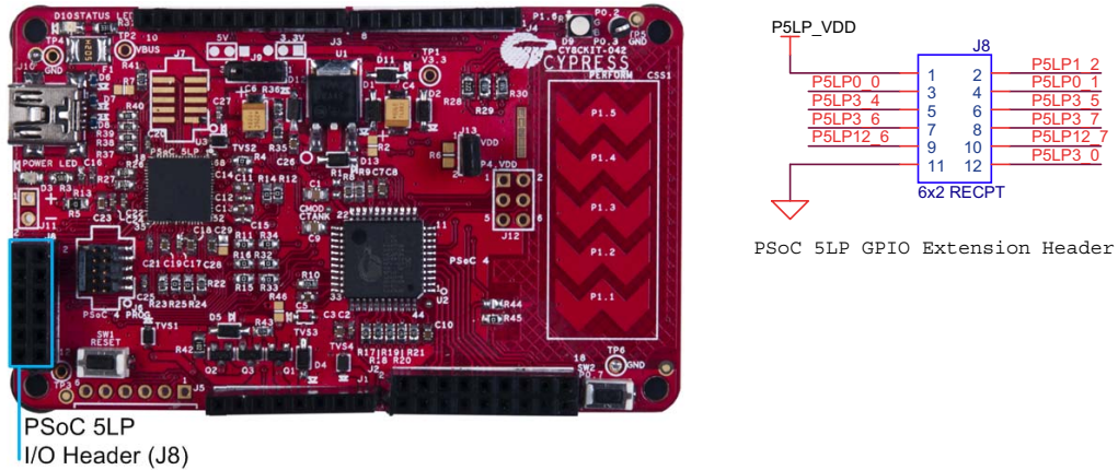
Figure 4-12. PSoc 5LP GPIO Header (J8)
