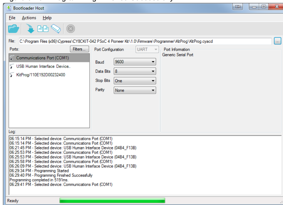
Figure 6-49. Programming Finished Successfully
