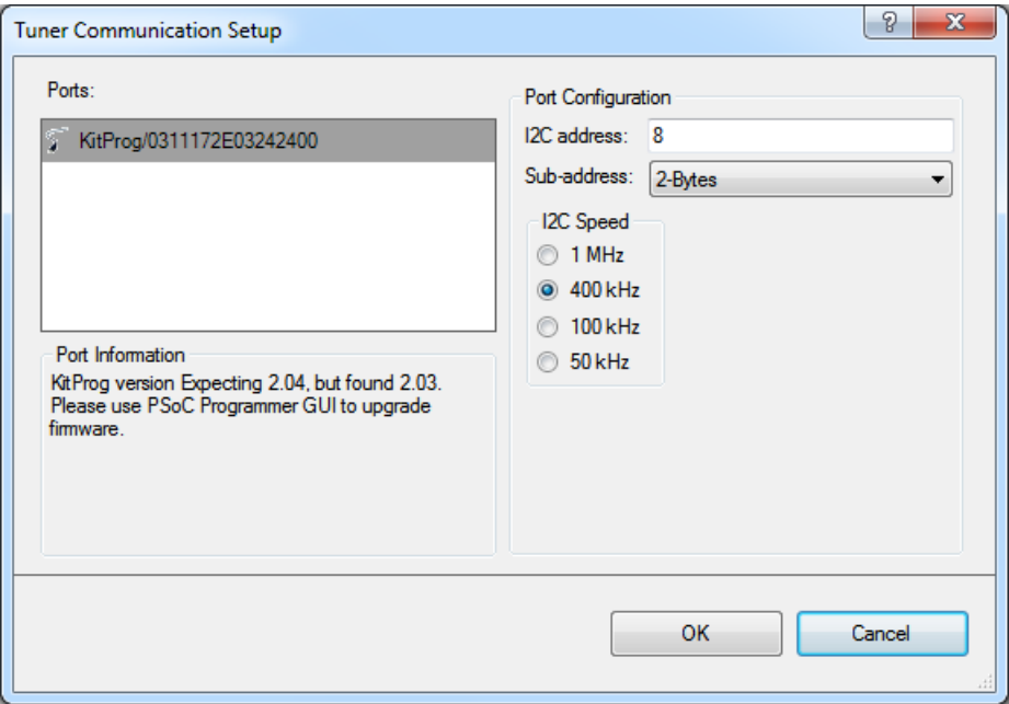
Figure 5-24. I2C Communication
