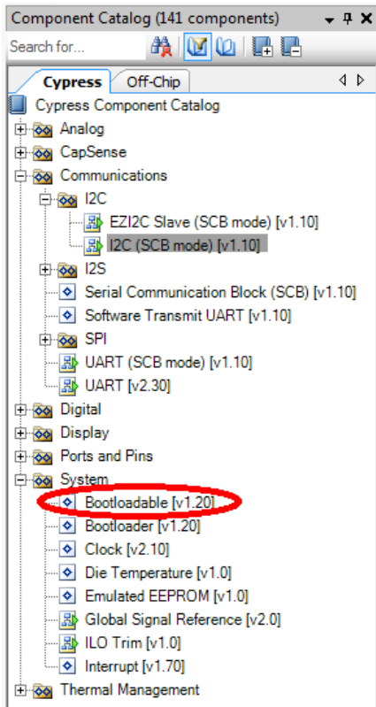
Figure 6-34. Bootloadable Component in Component Catalog
