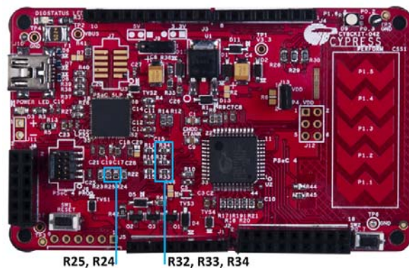
Figure 4-7. Zero-ohm Resistor Position
