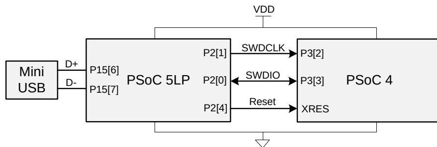
Figure 3-5. SWD Programming PSoC 4 Using PSoC 5LP
