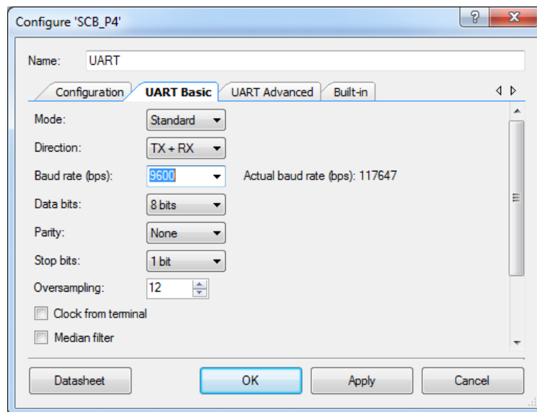
Figure 6-5. UART Basic Configuration Window
