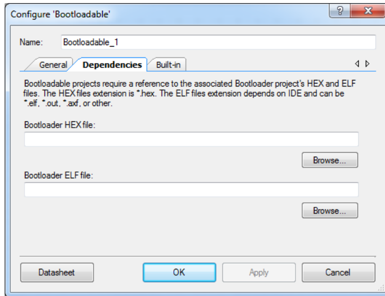
Figure 6-35. Configuration Window of Bootloadable Component
