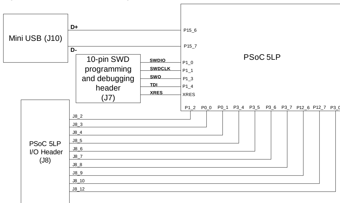
Figure 6-30. PSoC 5LP Block Diagram
