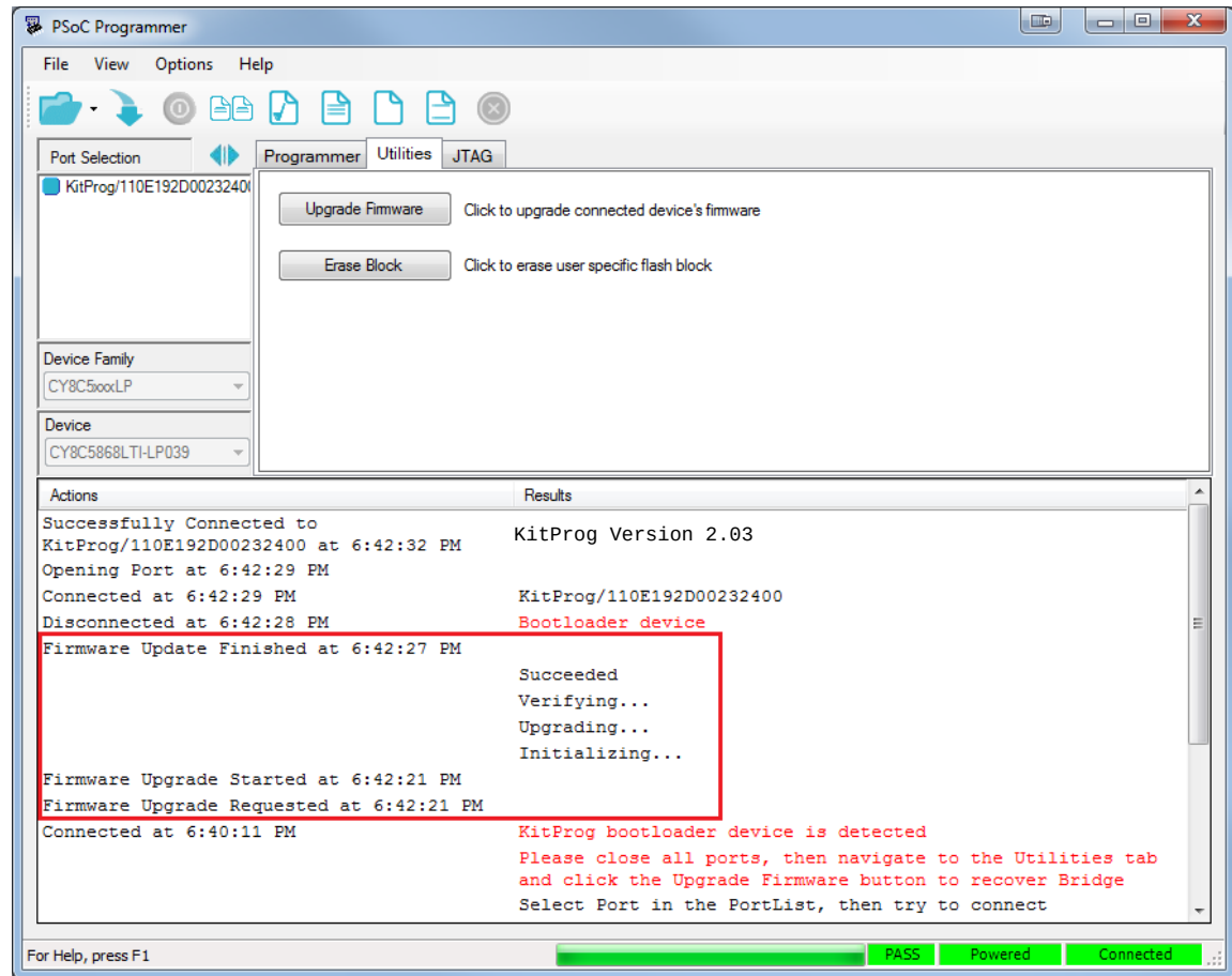
Figure 6-46. Firmware Update Complete
