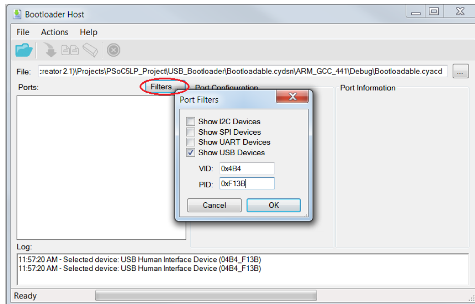
Figure 6-40. Port Filters Tab in Bootloader Host Tool
