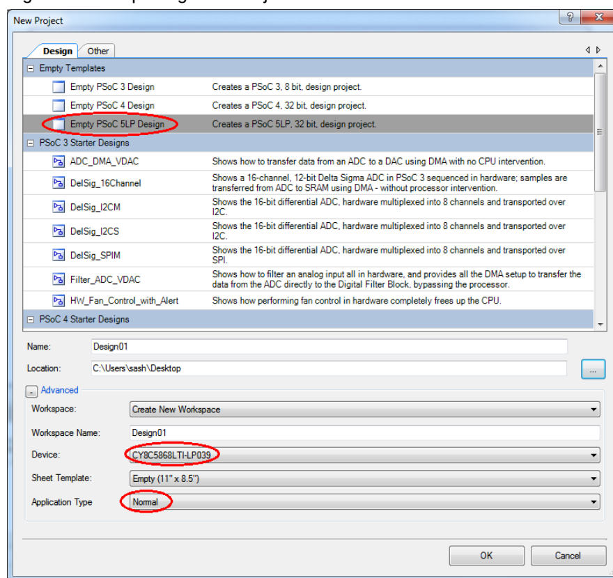
Figure 6-43. Opening New Project in PSoC Creator
