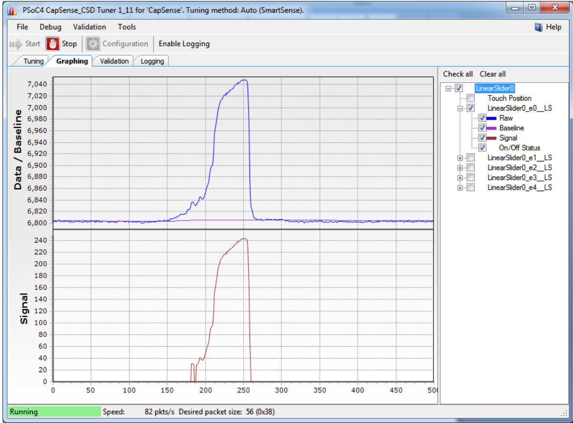
Figure 5-28. Raw Count Increase
