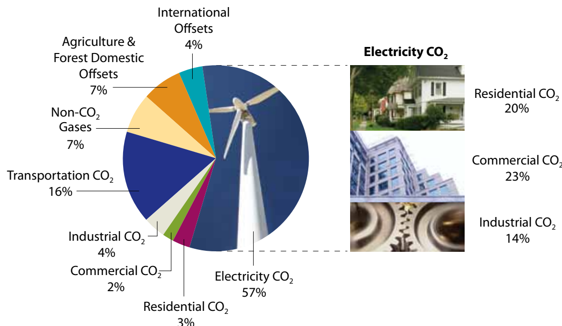
FIGURE ES.5. The Source of Cuts in Global Warming Emissions in 2030
